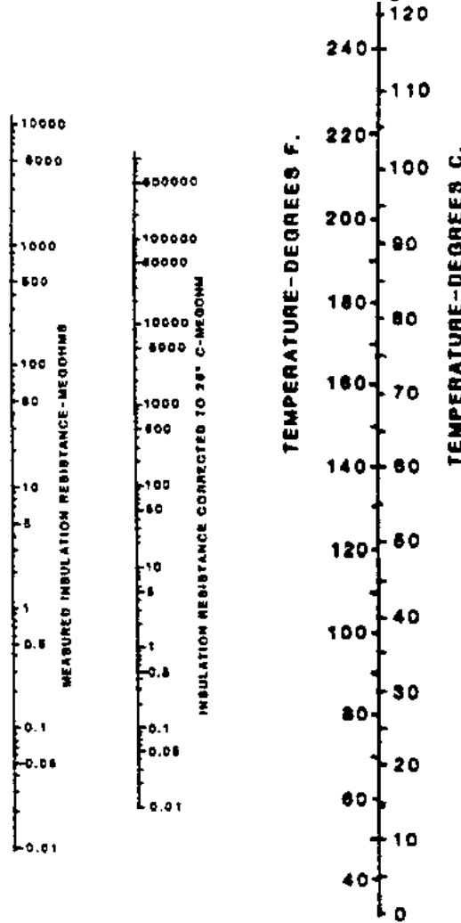
FIGURE 1 – INSULATION RESISTANCE TEMPERATURE CORRECTION NOMOGRAPH
