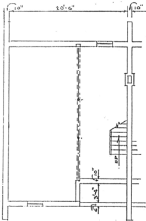
BASEMENT PLAN
