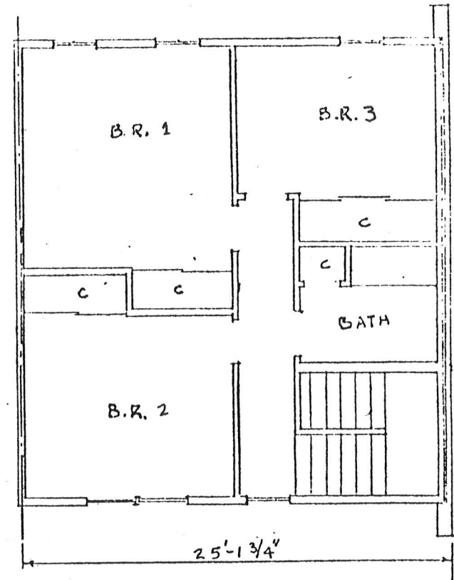
SECOND FLOOR
