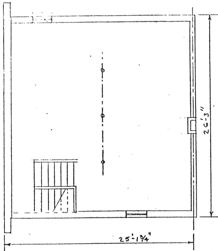
BASEMENT
